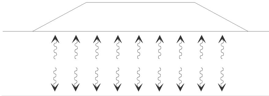
Fig. 4 – Consolidation without prefabricated vertical drains
