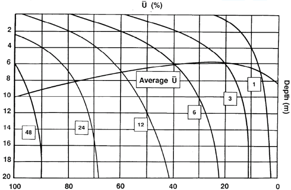
Fig. 7 –Effect of drain depth on consolidation time
